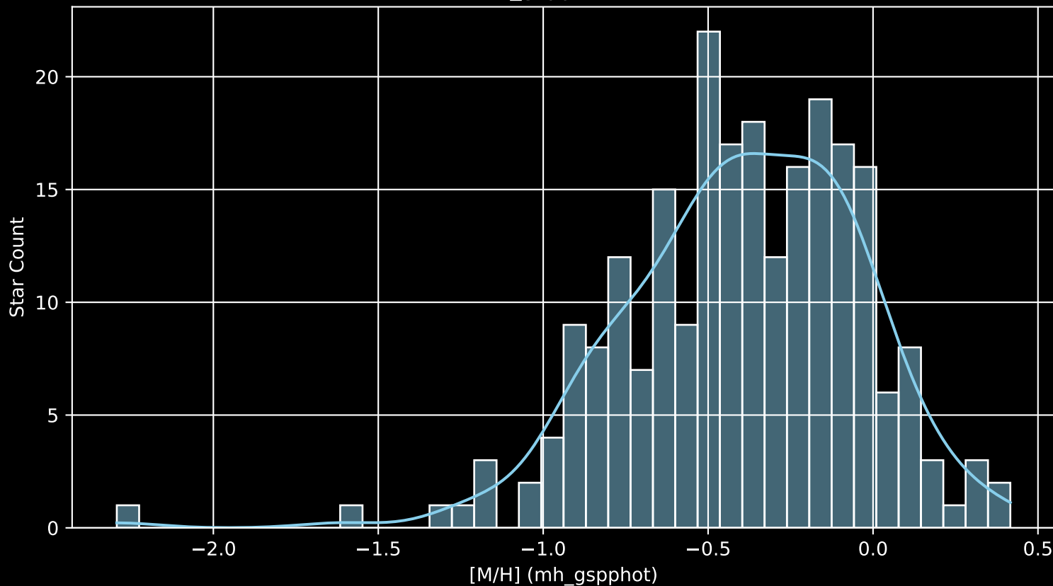
GALAH DR4 Field: [7226] [M/H] (mh_gspphot) (n= 233)
