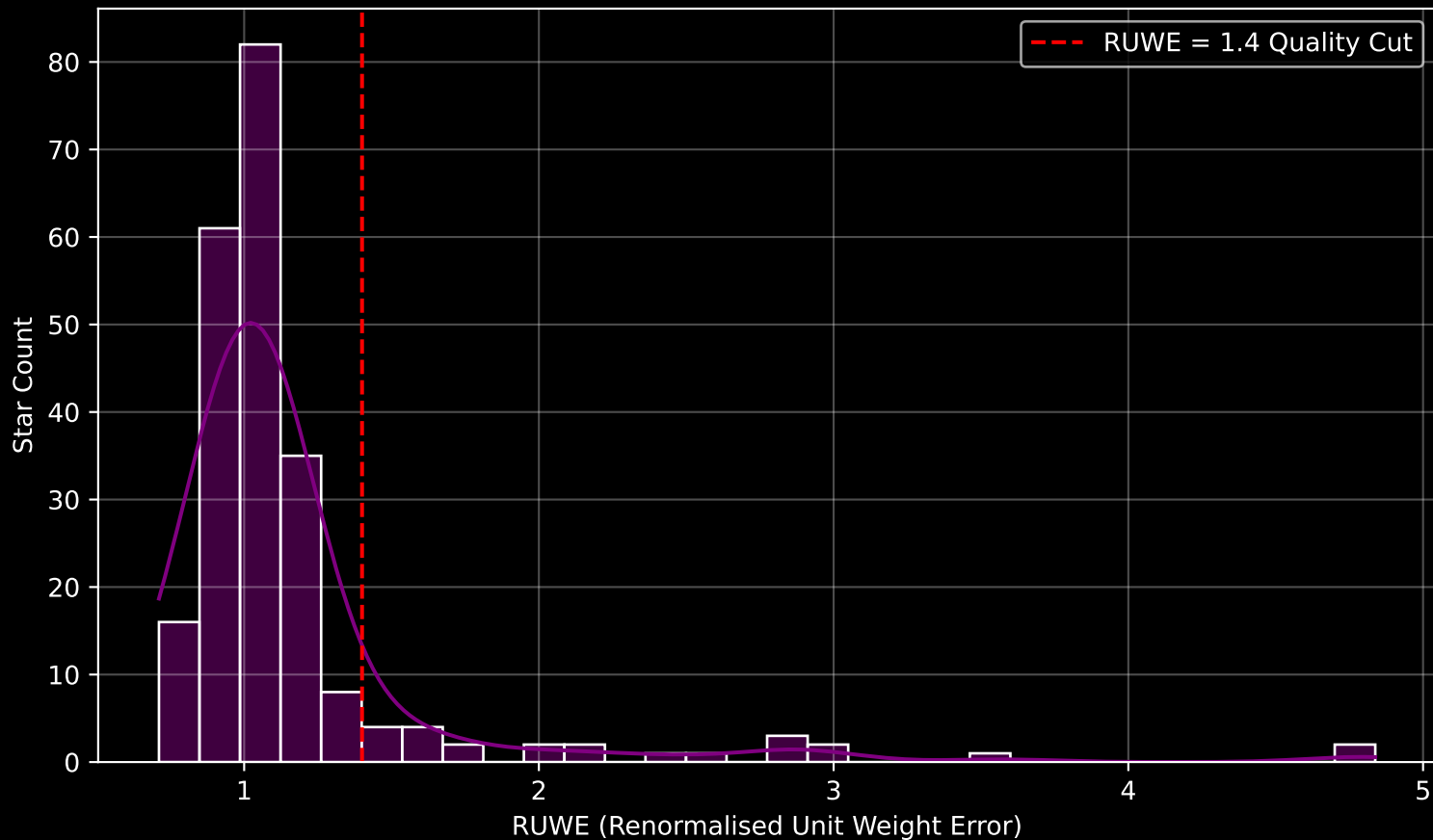
GALAH DR4 Field [7226] RUWE Distribution (n= 226)
