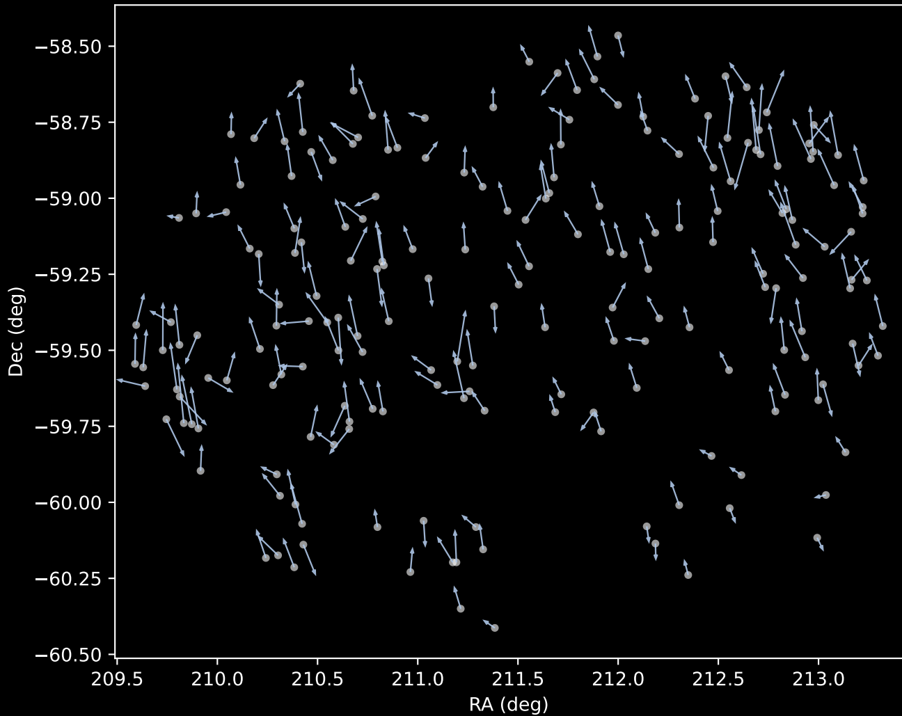
GALAH DR4 Cluster 1 Proper Motion Vectors (n=197)
