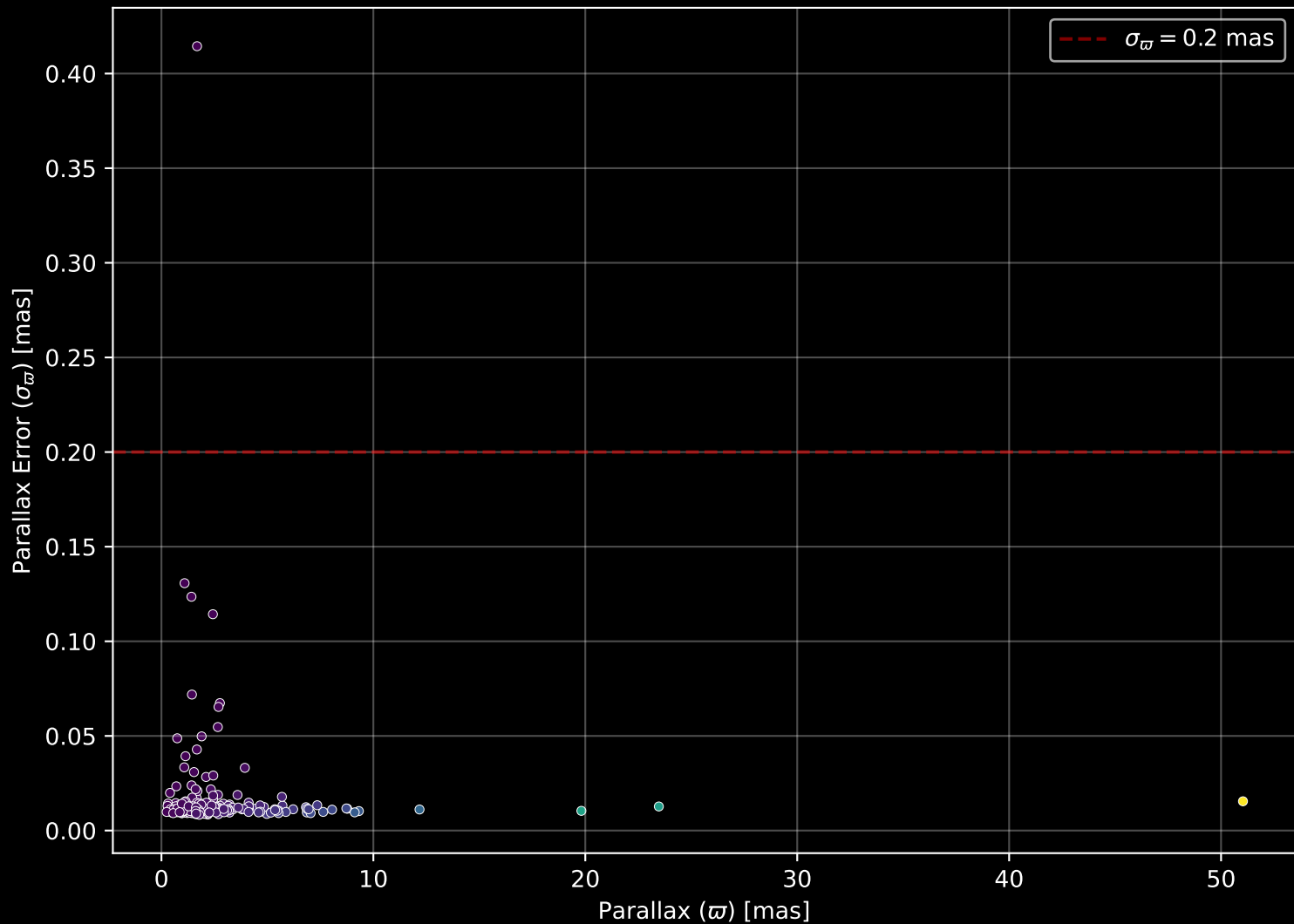
GALAH DR4 Field: [7226] Parallax Quality (n= 234)
