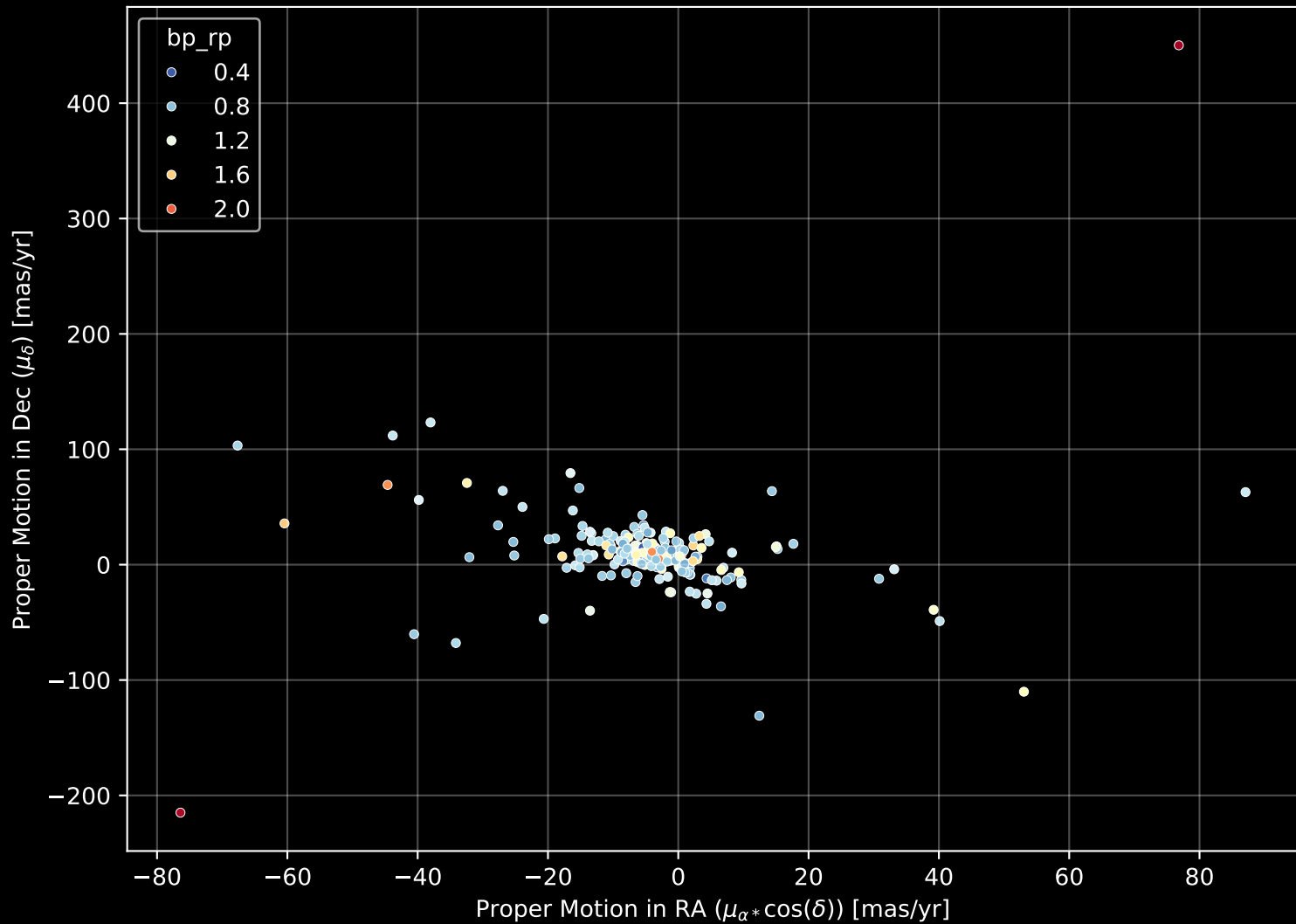
GALAH DR4 Field: [7226] Proper Motion Diagram (n= 234)
