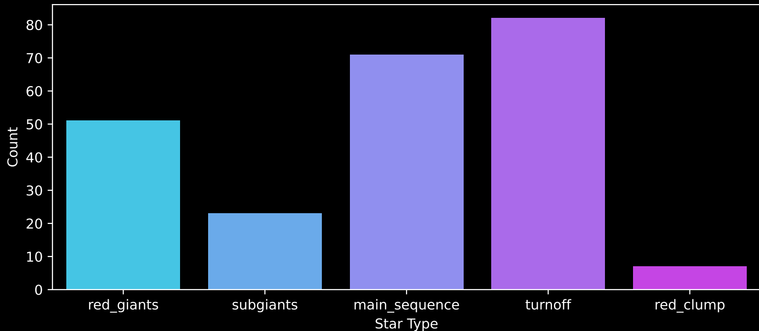
GALAH DR4 Field: [7226] Count plot of Star Type
